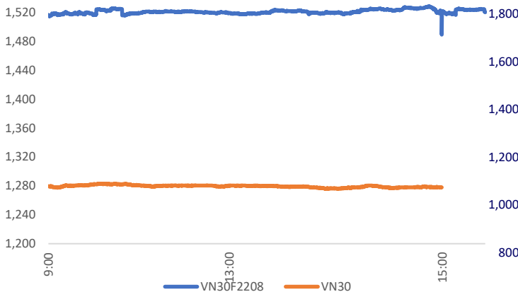
VN30F2207 & VN30 - INTRADAY
